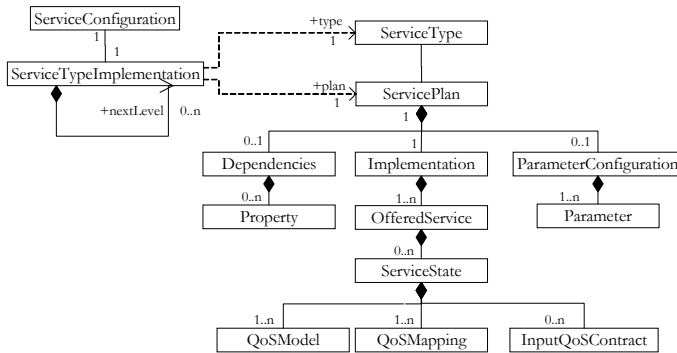
Fig. 6. Service Configuration
