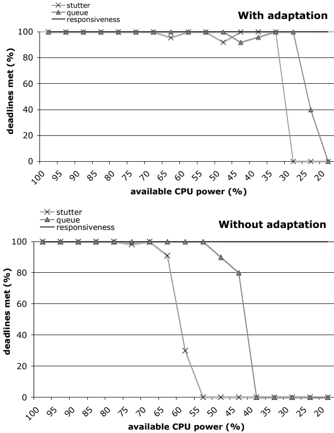
Fig. 8. Dale constraint violations with and without adaptation
