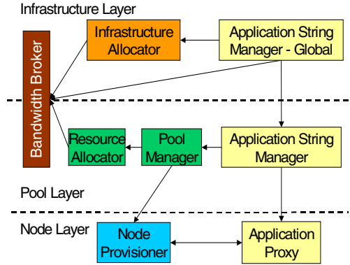
Fig. 1. Our fault-tolerance capability mirrors the layered structure of the MLRM architecture
