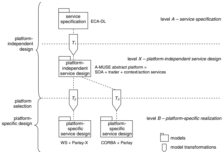
Fig. 3. Design trajectory consisting of three levels of models
