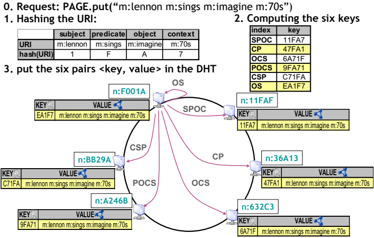
Fig. 1. Storing process
