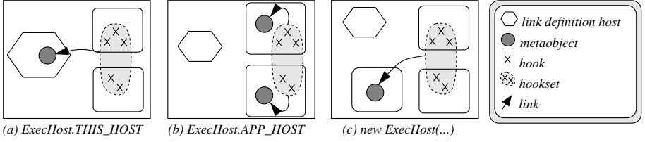
Fig. 3. Execution hosts
