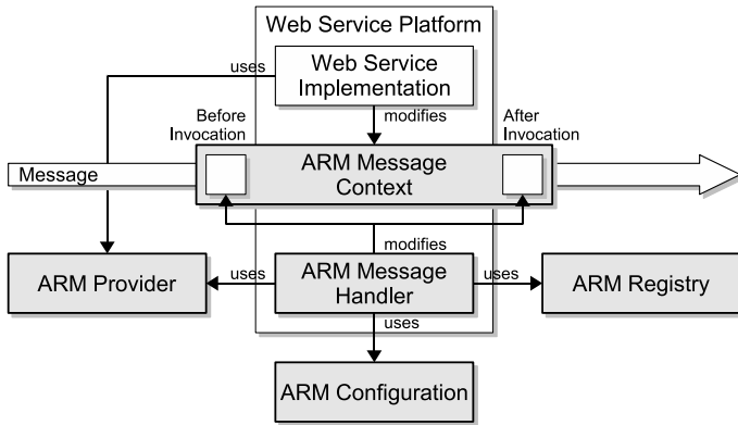
Fig. 3. Architectural Components
