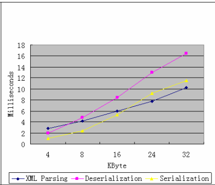
Fig. 3. Processing time on XML payload
