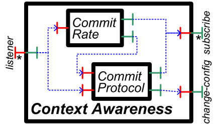
Fig. 10. Adaptation policy architecture
